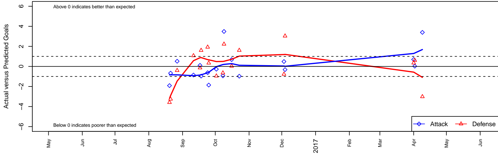
Beach FC South Bay Black B02 Dots are actual minus expected GF (blue circles) and GA (red triangles). Blue line is smoothed change in attack strength. Red is smoothed change in defense strength.
